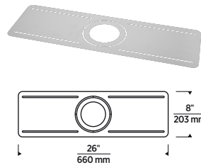
V-NCP NEW CONSTRUCTION PAN
