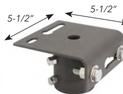
LF-AD-SF 2" slip fitter adapter for LF flood lights with trunnion. Goes on 2" pipe and accepts a trunnion fixture.
