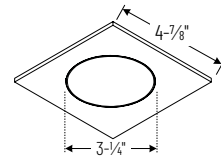
NIO-4SNDC Square Reflector with Round Aperture Non-Adjustable
