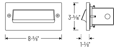
NSW-843/32 Shroud
