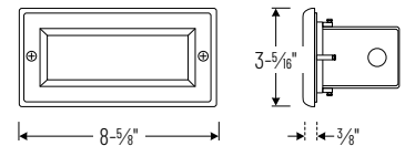
NSW-842/32 Lensed
